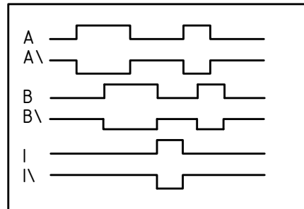
NT03 WITH LINE DRIVER OUTPUT SIGNALS
